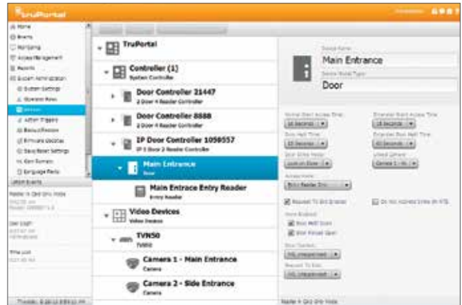
Device tree
