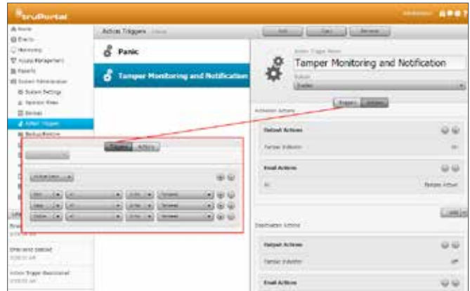
Action Triggers
